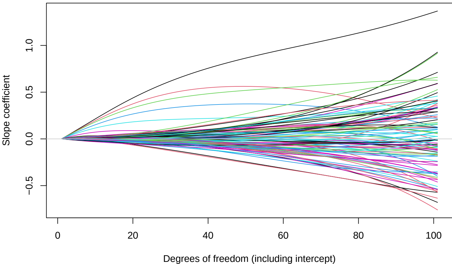
ridge coefficient path: p = 100
